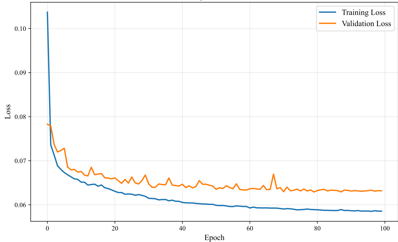
Bi-TSENet Training & Validation Loss - data8
